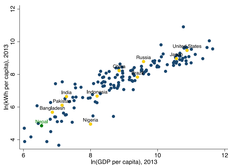
Figure 1. Electricity consumption is strongly correlated with economic development (Wolfram, 2016)
